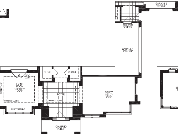
PART. GROUND FLOOR PLAN | Elevation C
