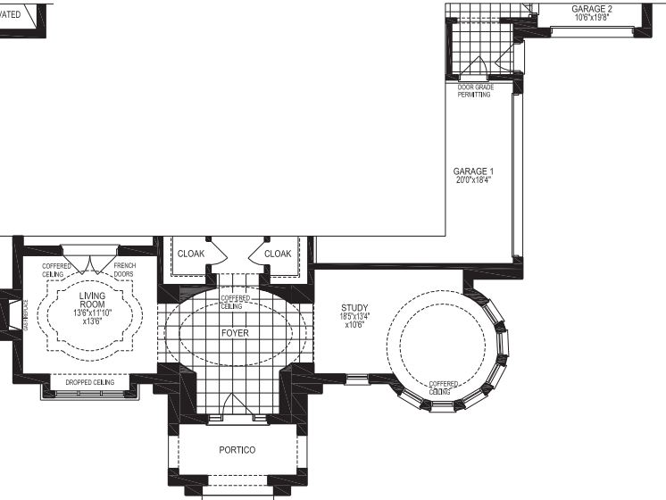
PART. GROUND FLOOR PLAN | Elevation B
