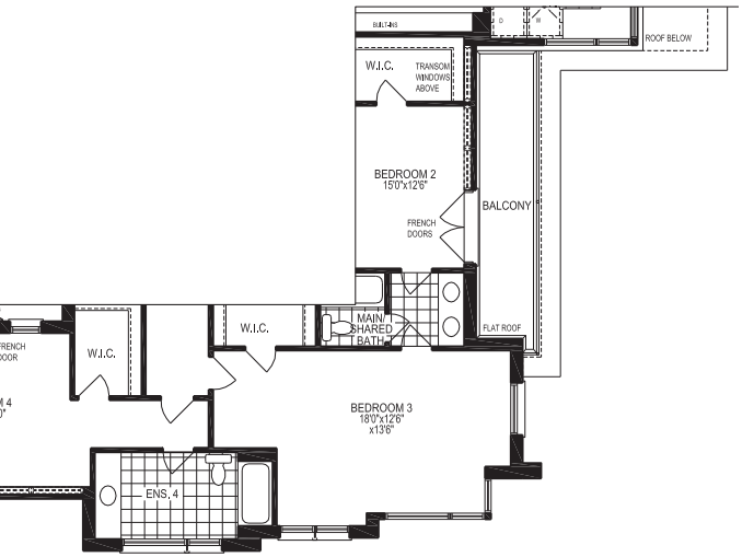
PART. SECOND FLOOR PLAN | Elevation C
