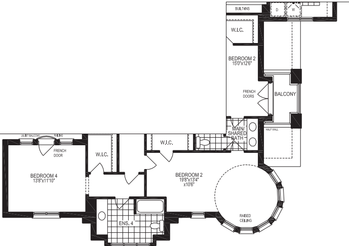
PART. SECOND FLOOR PLAN | Elevation B
